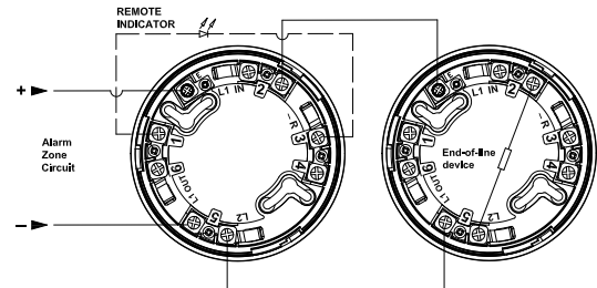
Fig. 1: 2-wire base wiring connections
